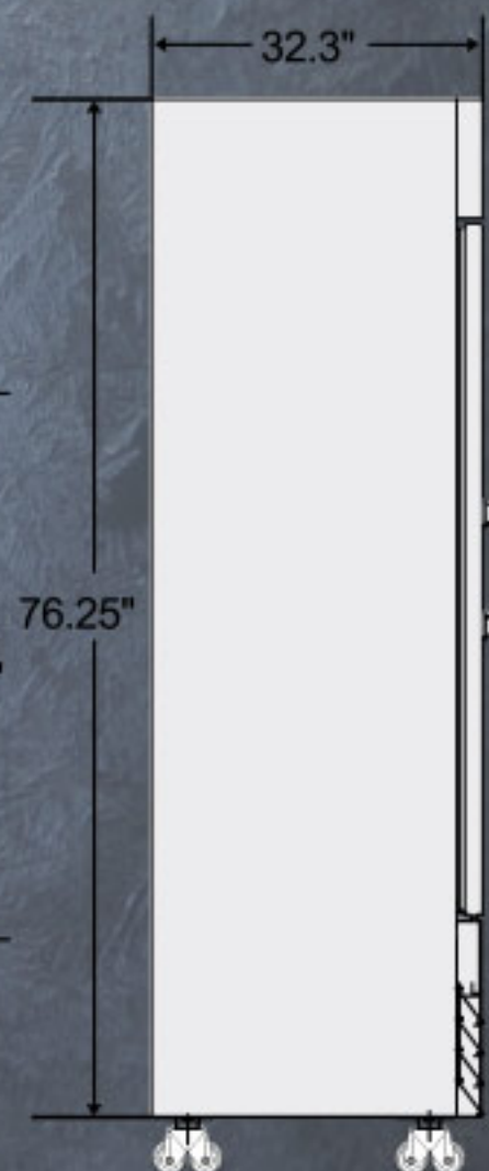
Side View
